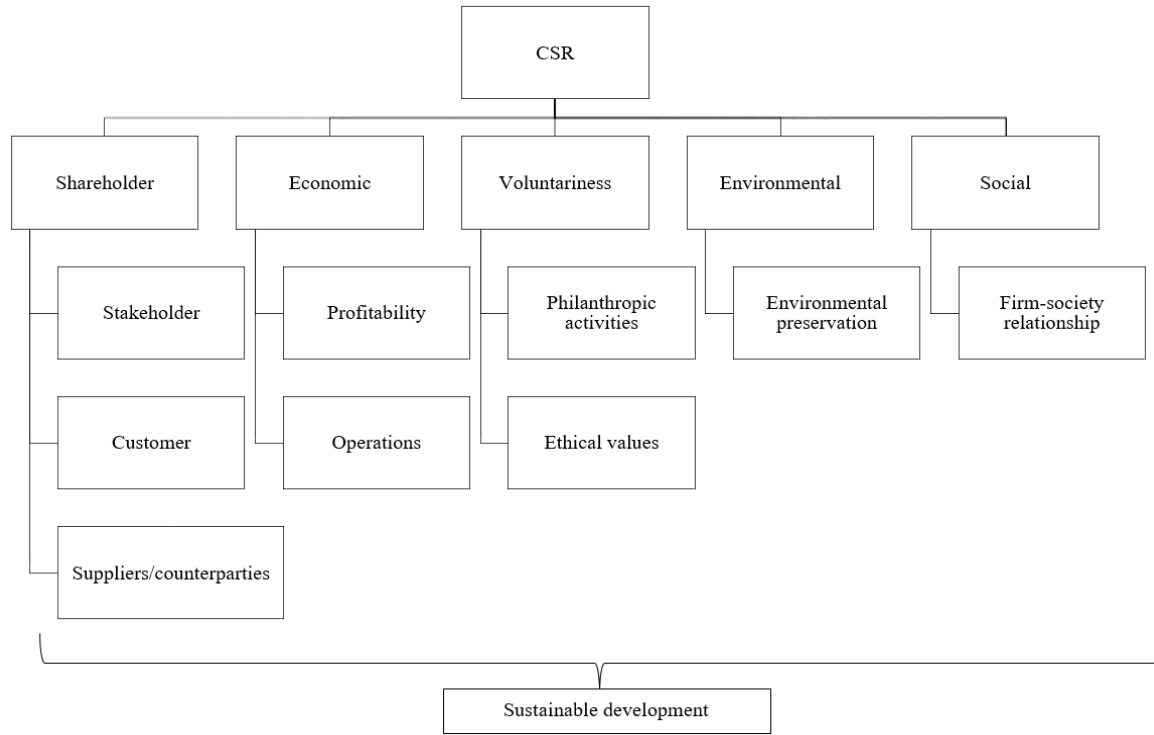
Figure 1. CSR Framework
