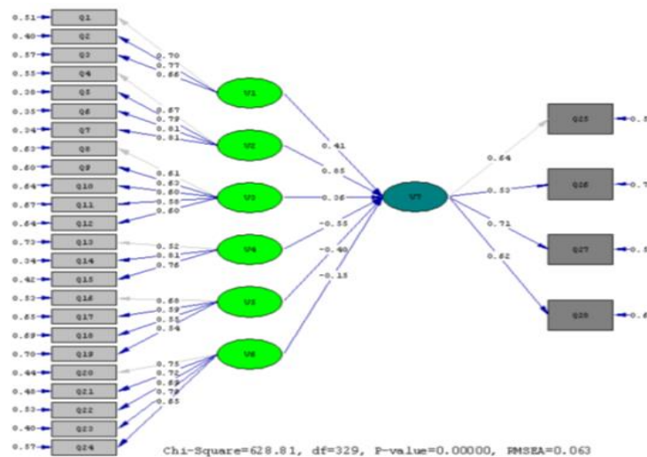
Figure 2. Standard Coefficients of Structural Model and Measurement
