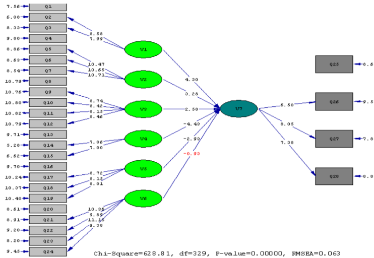
Figure 1. Statistics t for Structural Model and Measurement
